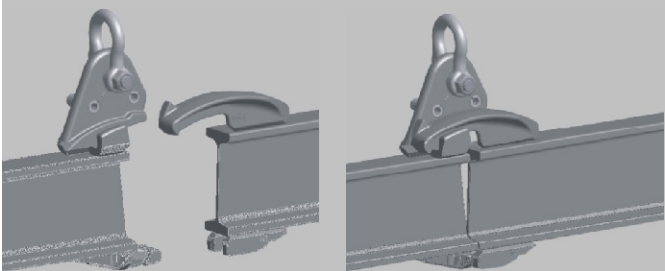
Insert rail (lug end) into rail (T-piece end)
